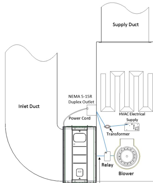
208V-480V input without EAC
