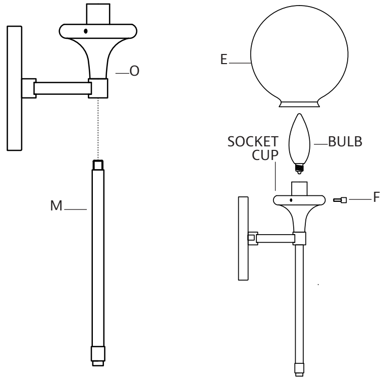
Installation (FIG. 2)
