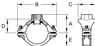
Figure 522 Sprinkler Outlet
