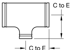
Figure 221 Cast Reducing Tee - Grooved
