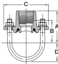
Figure 40-5 Strap (Pipe Outlet)
