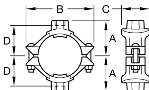
FIGURE 730 CROSS THREADED OUTLET
