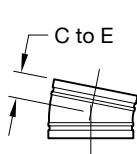
FIGURE 211, 311, & 511 FABRICATED 11-1/4° ELBOW (SEGMENT WELDED)
