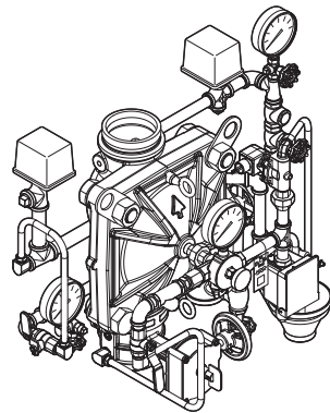
Electric Actuation Shown
