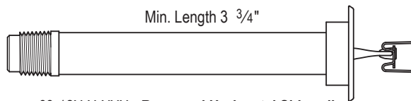
63-12X-X-XXX Recessed Horizontal Sidewall w/Std. Escutcheon (1" NPT)
