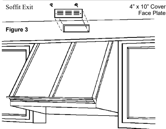
Soffit Exit
