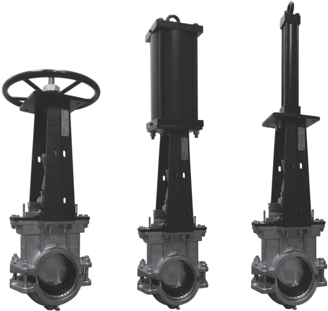
Series 906 Knife Gate Valve for Plain-End HDPE Pipe
