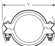
Style 995 14–20-inch sizes 350–500-mm sizes
