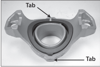
Style 920 Gasket
