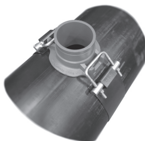
Style 926 Mechanical-T Spigot
