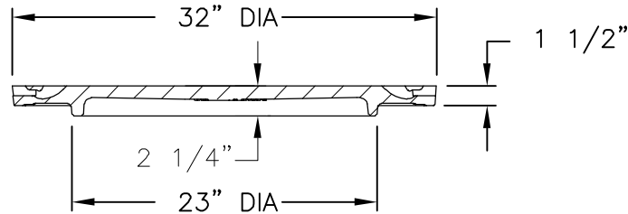
COVER SECTION
