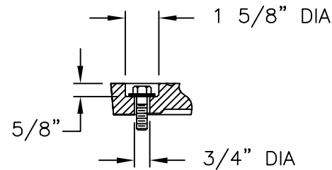
BOLTING DETAIL
