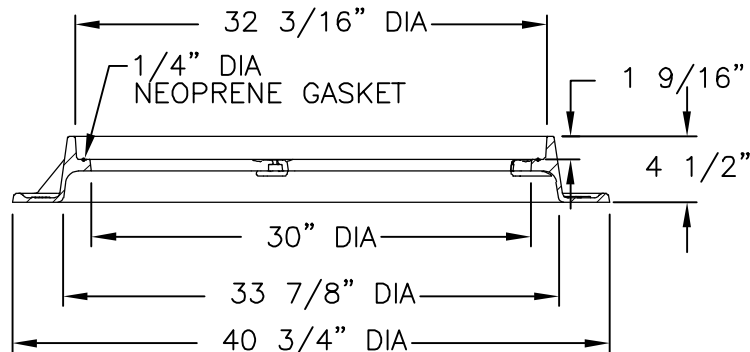
FRAME SECTION
