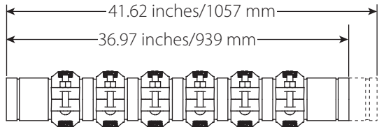
4-inch/DN100 Style 355/355P Expansion Joint
