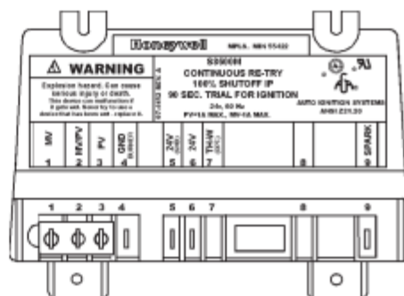
IGNITION MODULE FIGURE 3.
