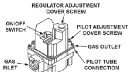
NATURAL VALVE
