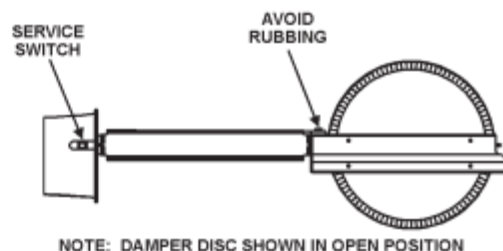
FLUE DAMPER FIGURE 4.
