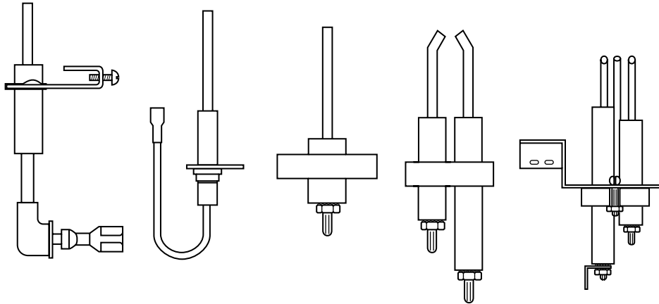
TYPICAL ELECTRODE ASSEMBLIES
