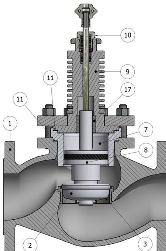
BEALANCED TRIM VALVE WITH FINNED BONNET
