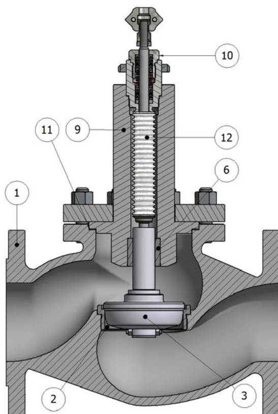
VALVE WITH BELLOWS
