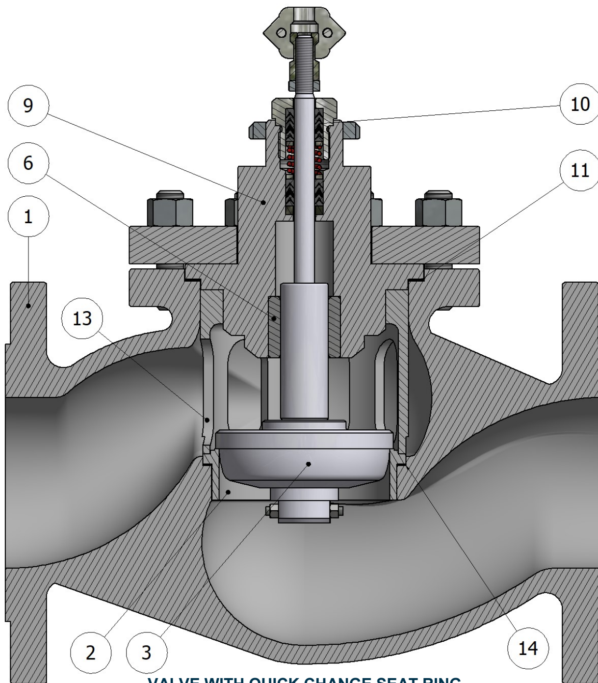
VALVE WITH QUICK CHANGE SEAT RING
