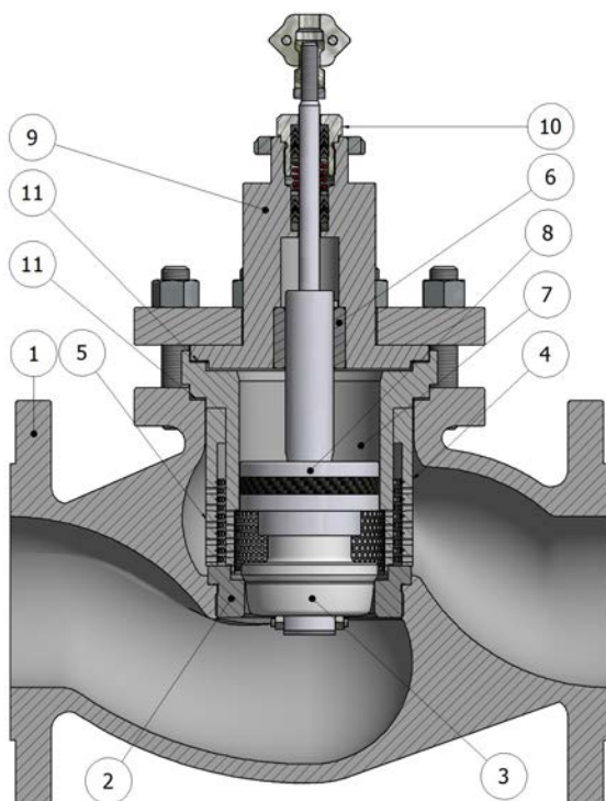
BEALANCED TRIM VALVE WITH DOUBLE CAGE NOISE REDUCTION
