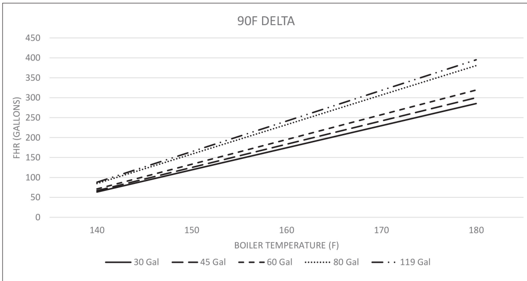
Figure 4 - 90F Delta
