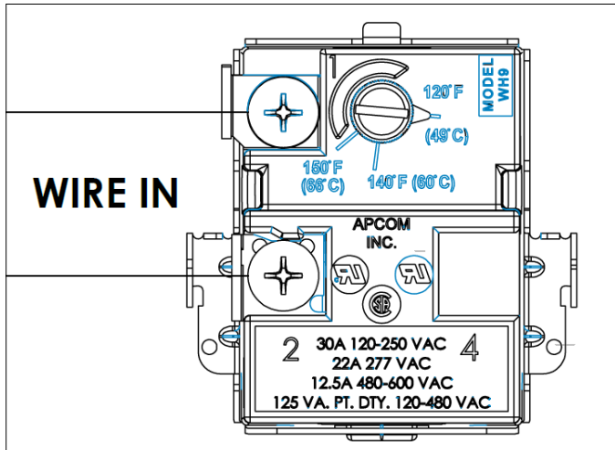
Figure 16 - Thermostat Connection
