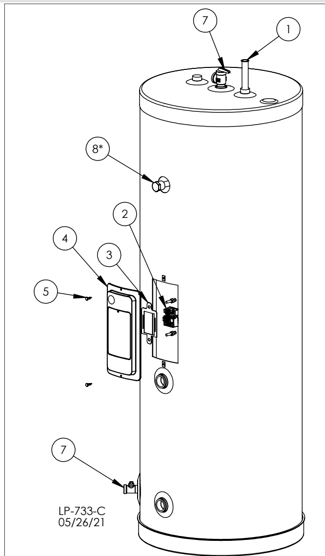
Figure 26 - Replacement Parts
