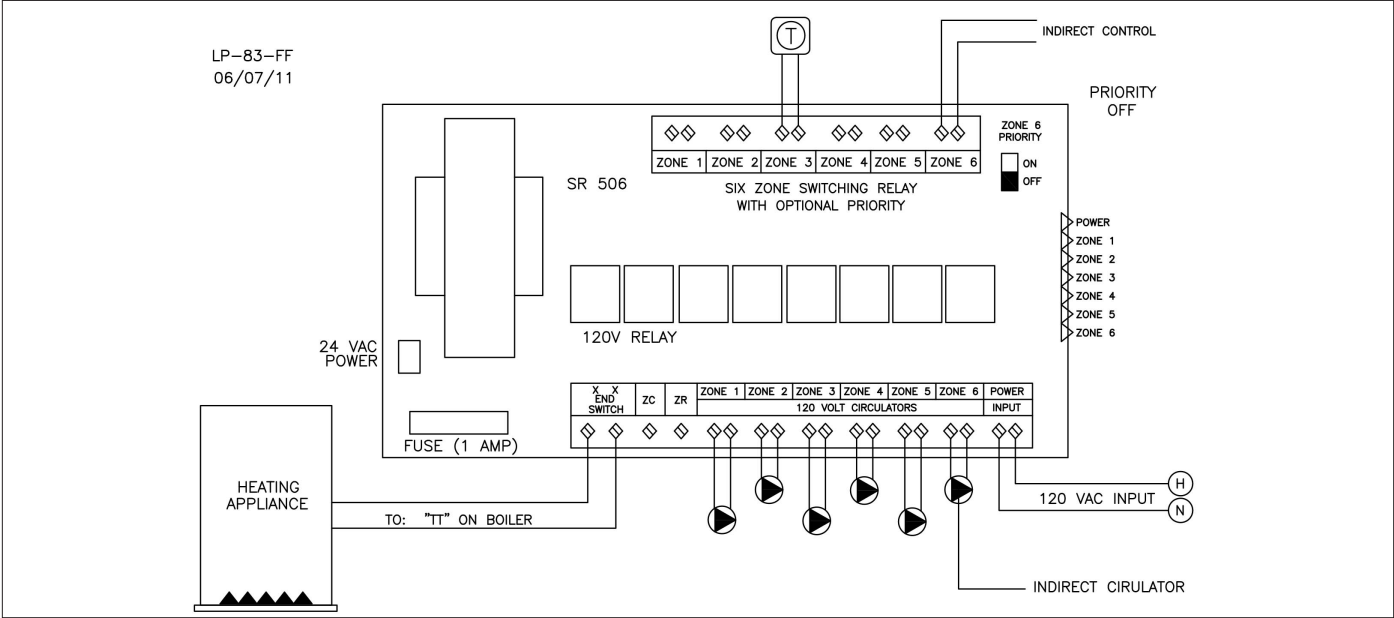
Figure 24 - Wiring with Circulators
