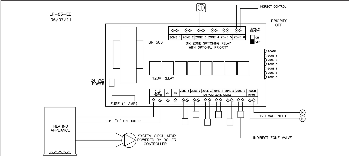
Figure 25 - Wiring with Zone Valves
