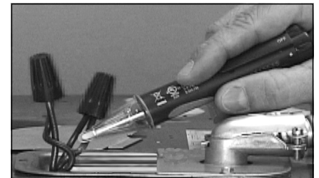
Figure 37 - Non-Contact Circuit Tester
