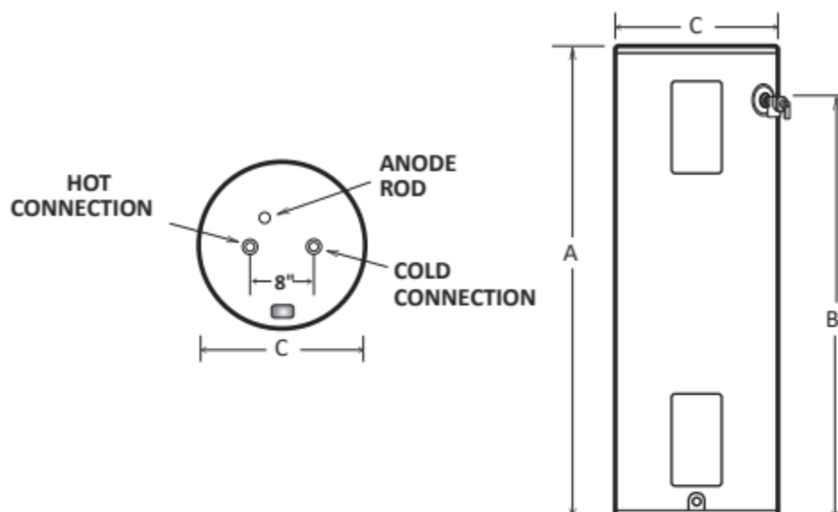
Figure 2. Rough-in Dimensions
