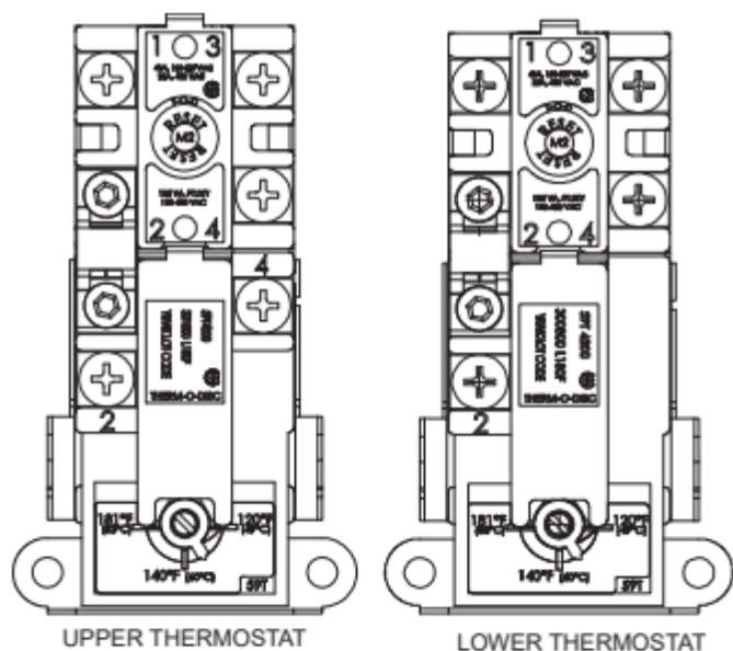
Figure 3. Thermostat Controls
