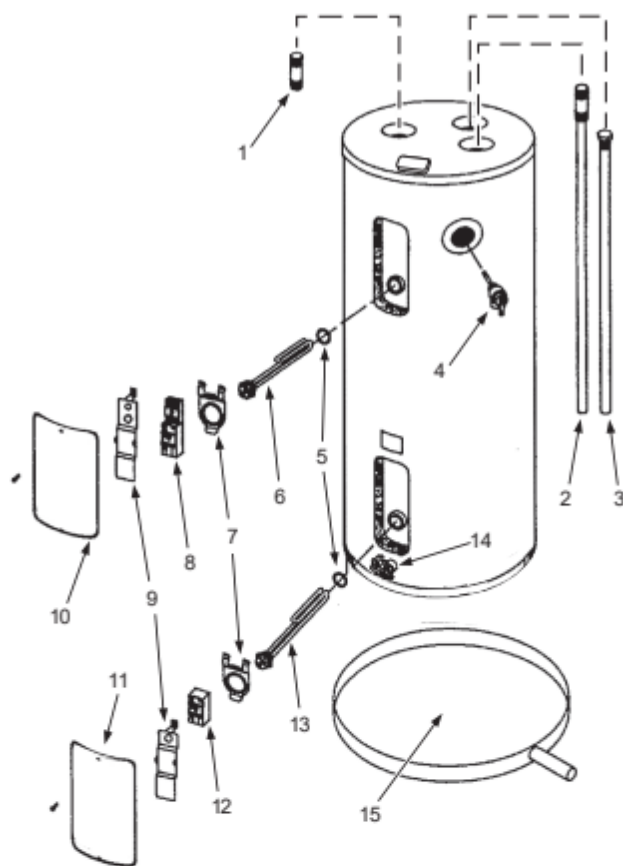
Figure 7. Repair Parts
