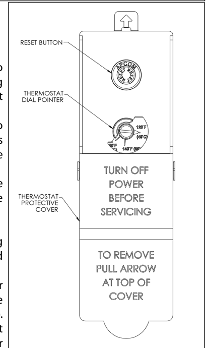
Figure 11 - Detail of Step #4
