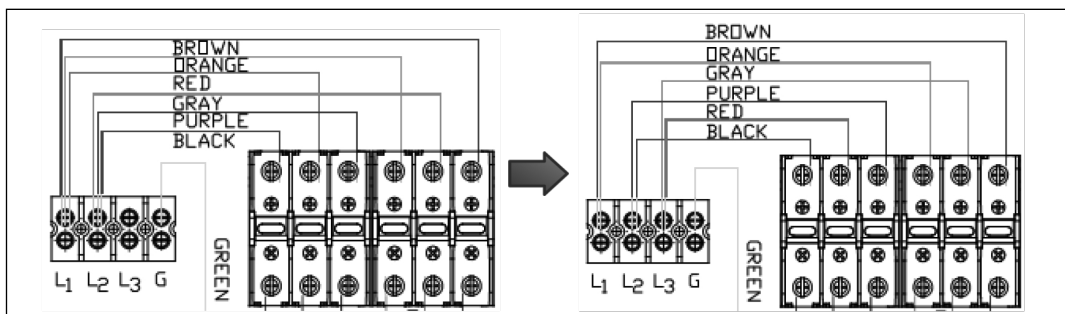
Figure 4 - Converting from Single to 3 Phase Operation
