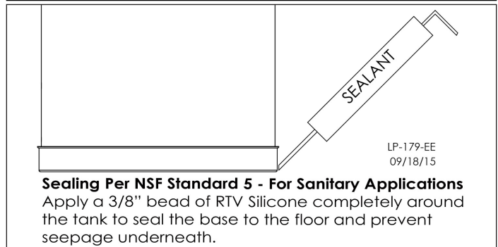
Figure 9 - Sealing the Water Heater for Sanitary Applications
