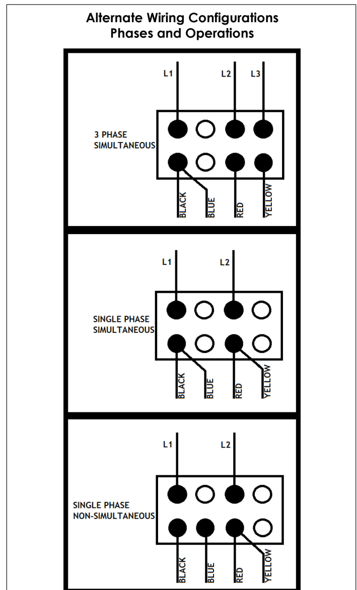
Figure 5 - Alternate, Field Installed Wiring Configurations, Single and Three Phase, Simultaneous and Non-Simultaneous Operation
