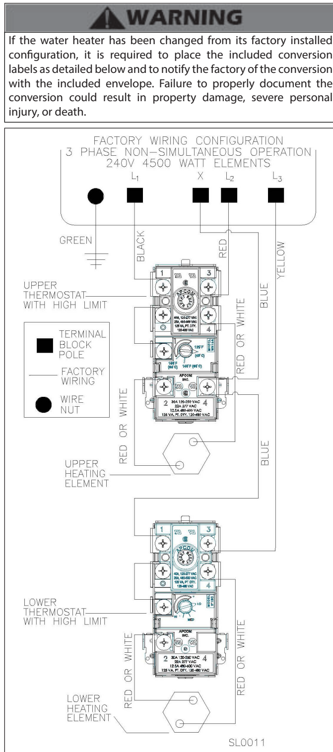
Figure 6 - Factory Installed Wiring Detail, 3 Phase, Non-Simultaneous Operation
