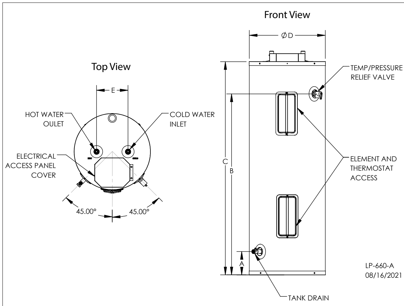
Figure 2 - Dimensional Drawing
