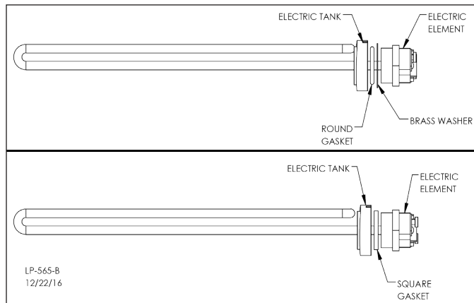
Figure 8 - Heating Element Detail
