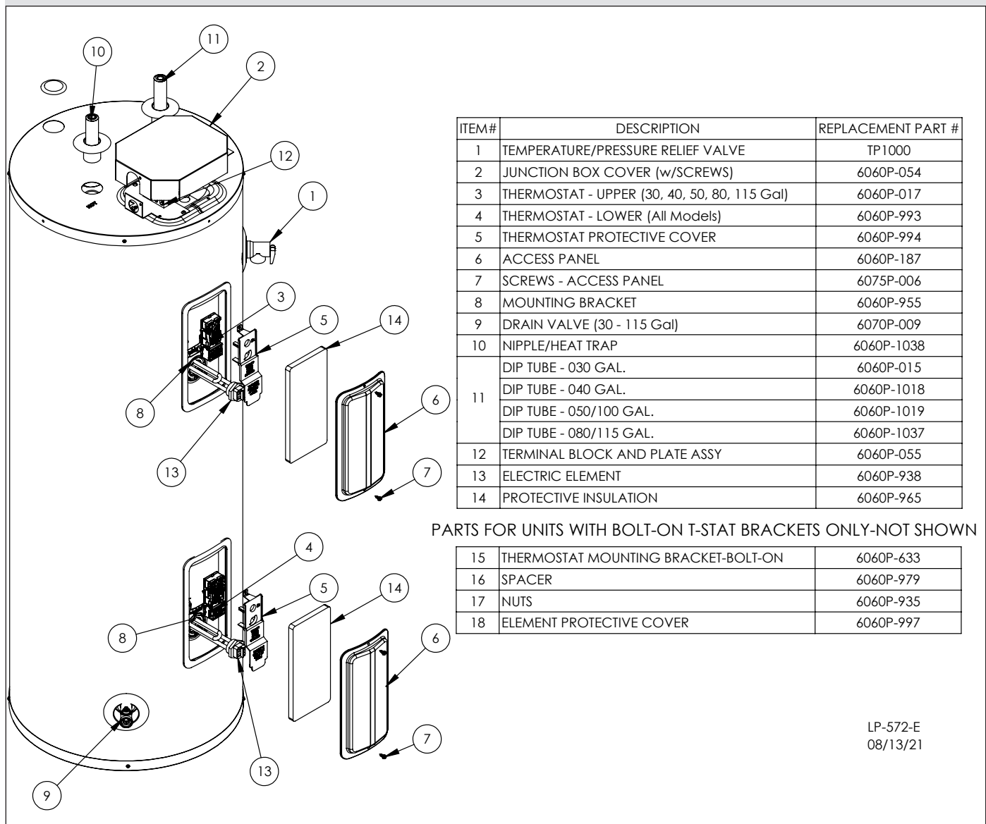
Figure 10 - Replacement Parts
