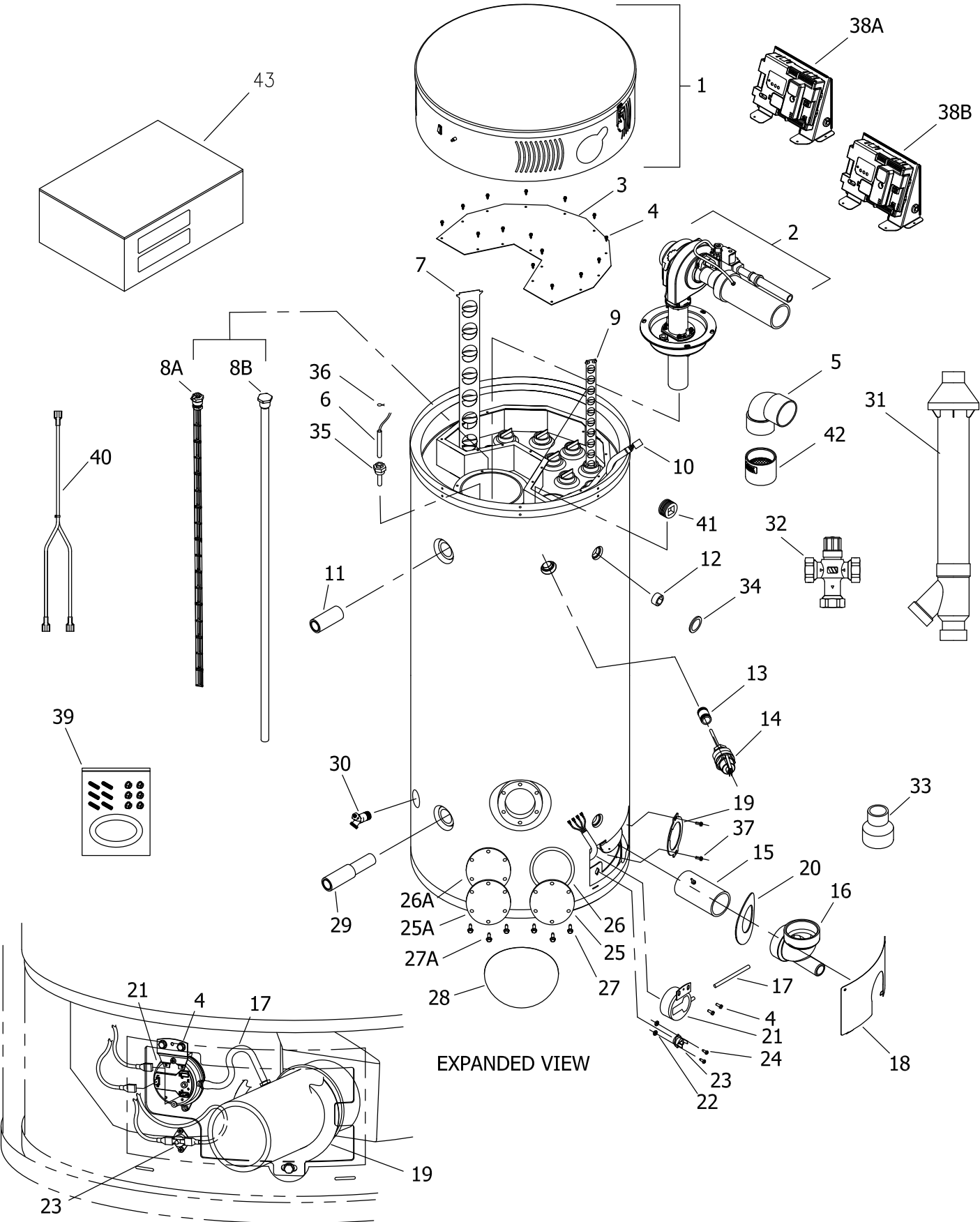
EXHAUST SERVICE AREA DETAIL (ASSEMBLED)
