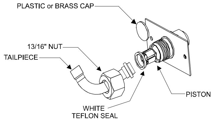
Figure 8 Flowrator
