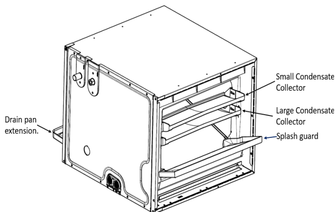
Figure 5 Horizontal Right Accessories Shown
