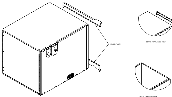
Figure 10 Block-off Plates & Duct Flange Detail
