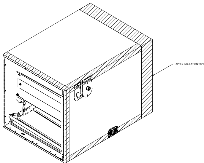
Figure 13 Panel Gap Sealing
