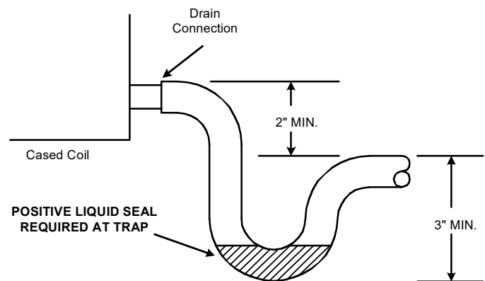
Figure 7 Condensate Drain Trap
