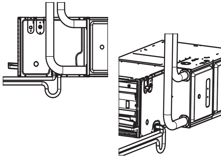
Figure 11 90% Flue Vent & Drain Port
