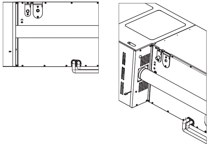
Figure 12 80% Flue Vent & Drain Port
