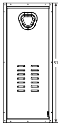
Recess Box for New Construction: 100306285
