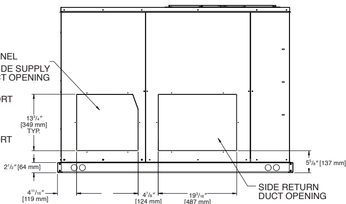
REAR VIEW
