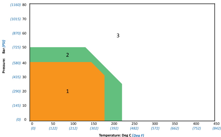
L430 PRESSURE / TEMPERATURE GRAPH
