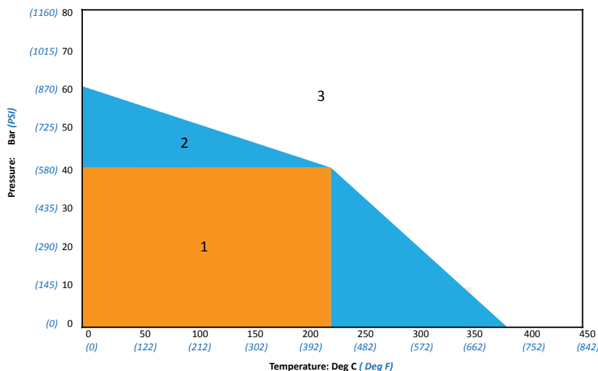
L441 PRESSURE / TEMPERATURE GRAPH
