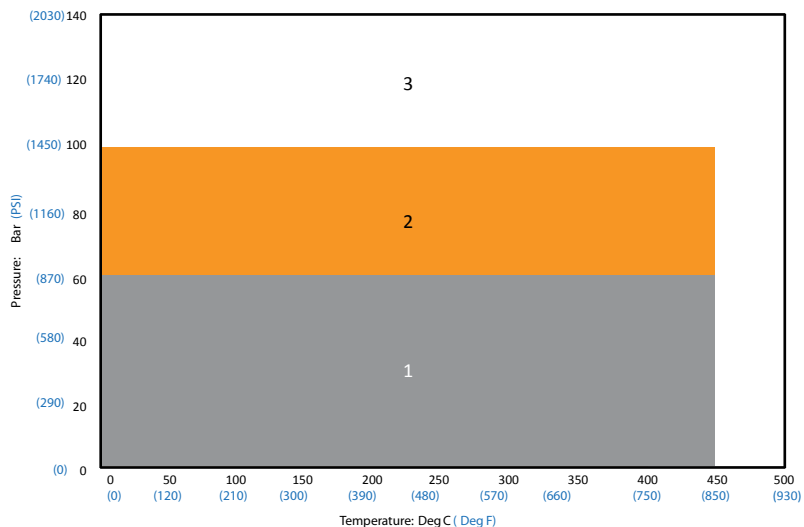
LG-SS PRESSURE / TEMPERATURE GRAPH
