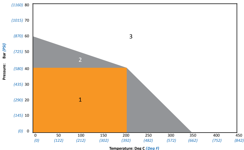
L640W PRESSURE / TEMPERATURE GRAPH
