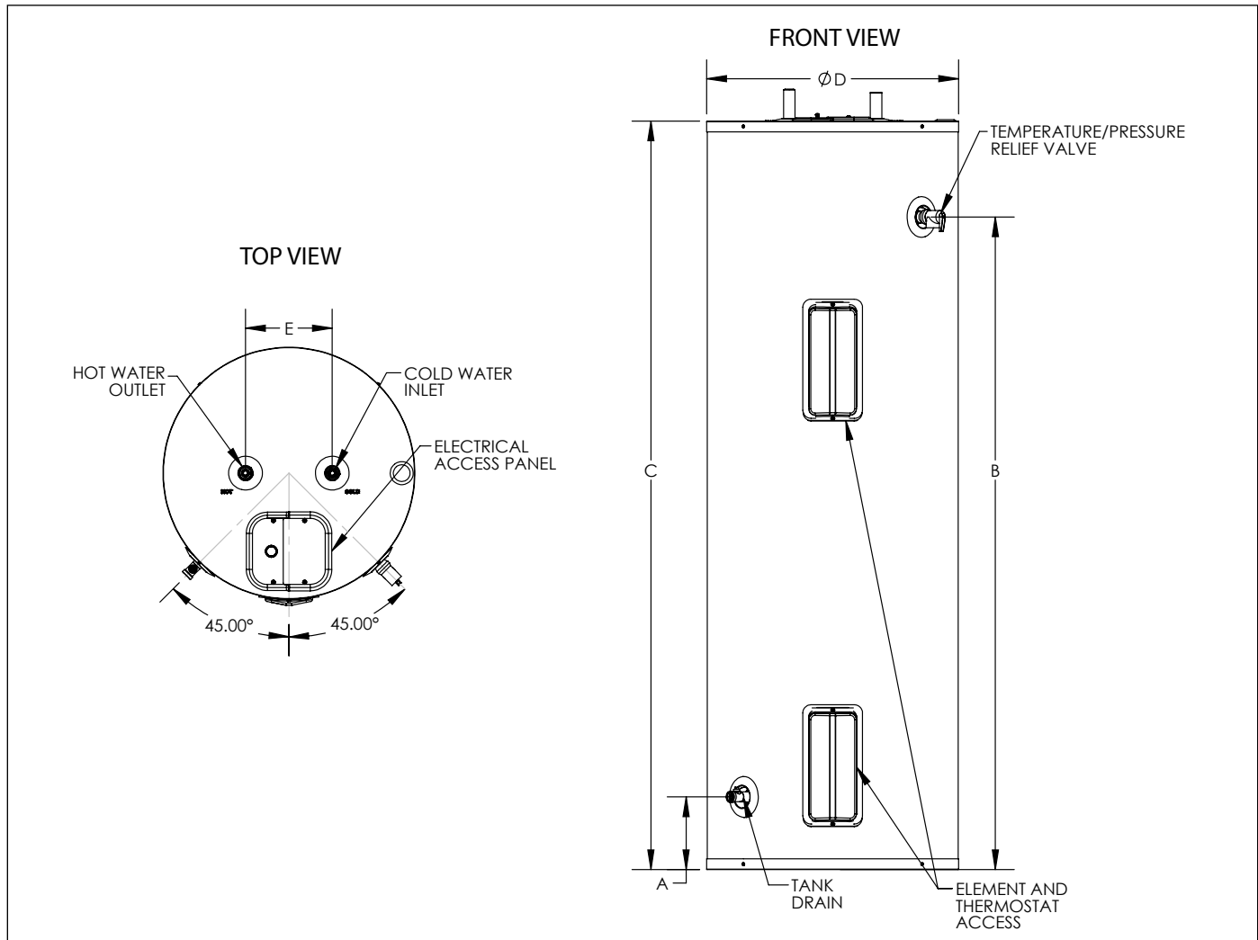
Figure 2 - Dimensional Drawing
