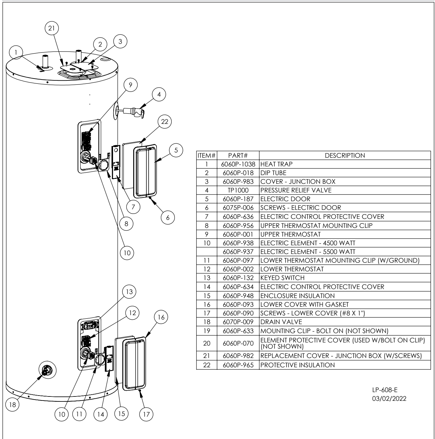
Figure 8 - Replacement Parts
