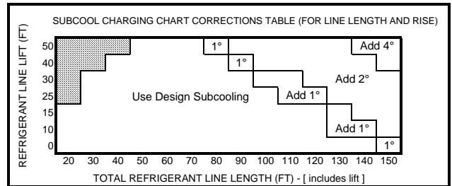
Figure 7. 5.0 Ton Models
