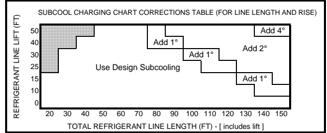
Figure 6. 4.0 Ton Models
