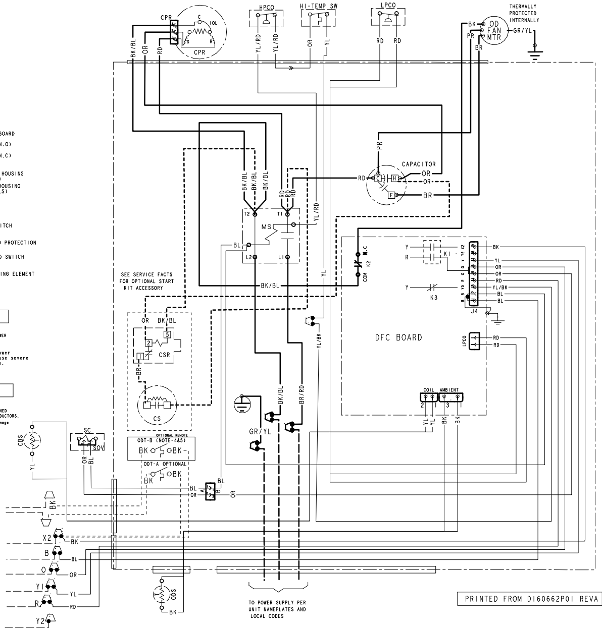
Figure 2. 3.0 Ton Models
