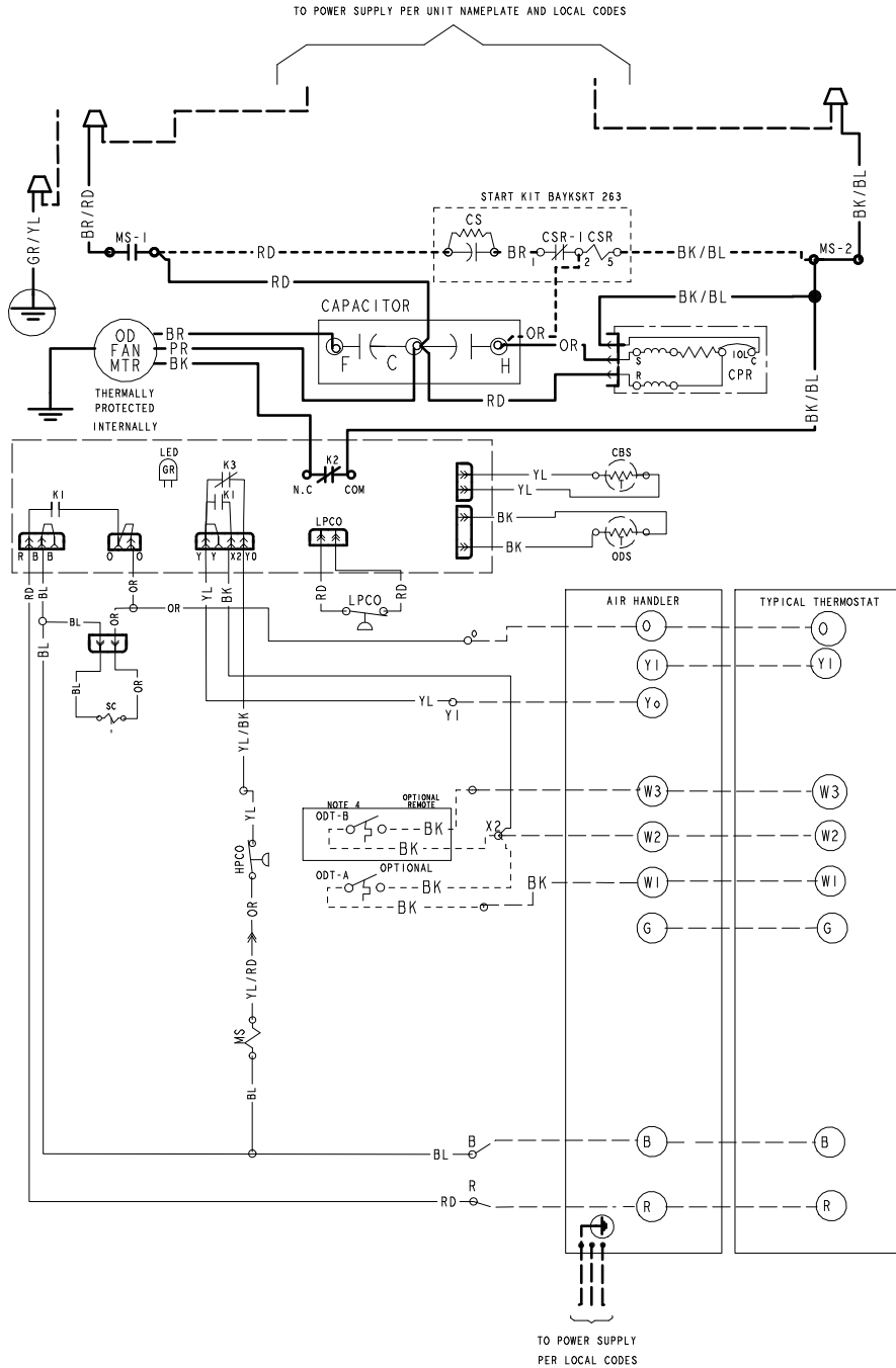
Figure 1. 3.0 Ton Models
