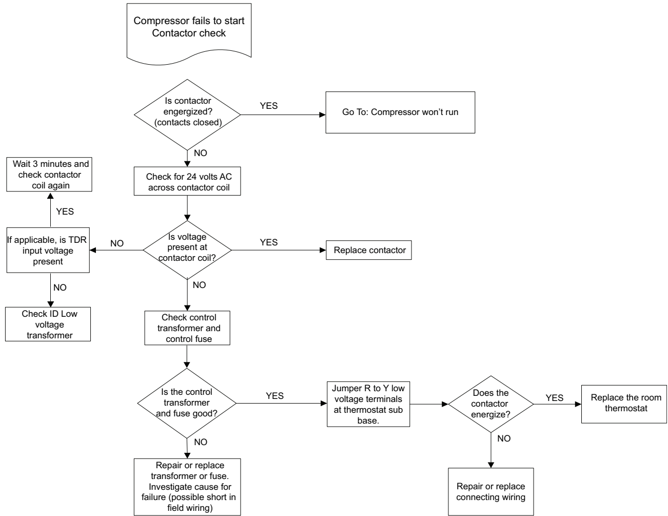
Single Pole Contactor (MS)*
