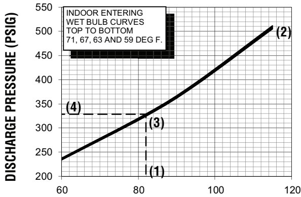
OUTDOOR TEMPERATURE (Degree F)
