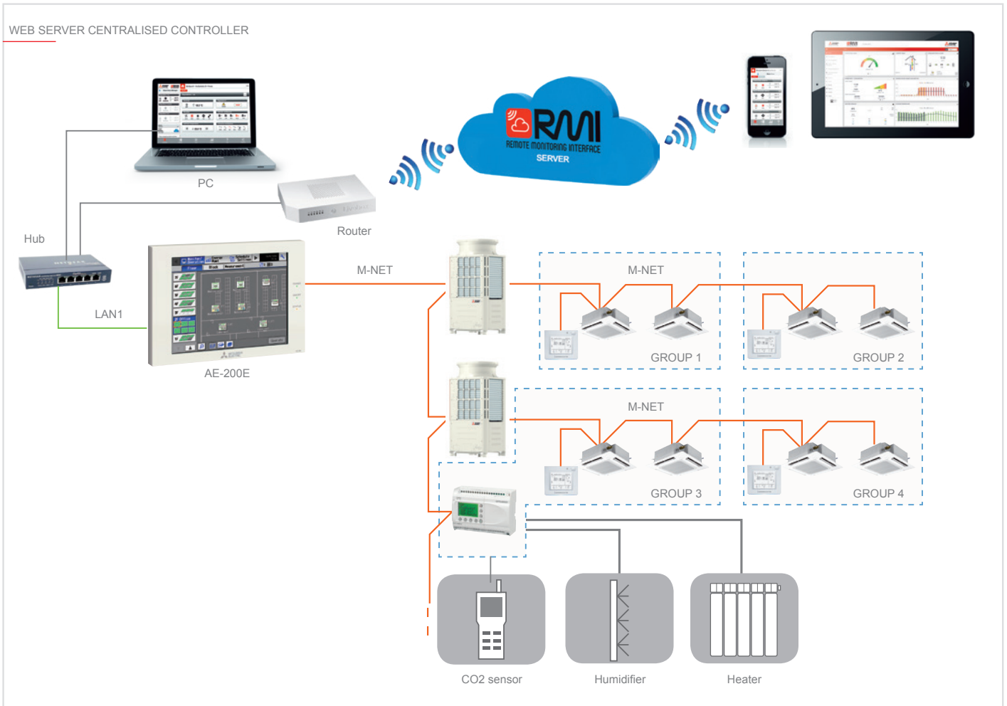
WEB BROWSER MONITORING AND CONTROL FUNCTIONS
