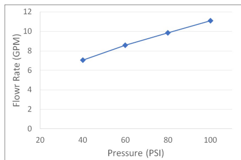
P-1131B Flow Rate (GPM) Vs Pressure (PSI) For Tub Port*
