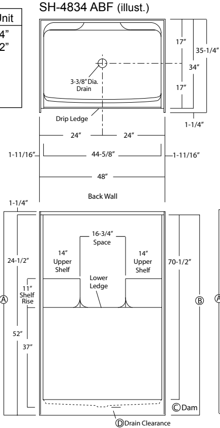
Illustration 1b - Center Drain, Unit Dimension & Alcove Framing Guidelines (dimensional tolerance +/- 1/8")
