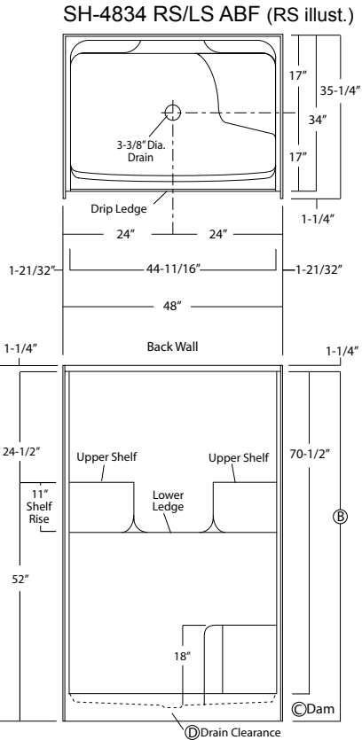
Illustration 1b - Center Drain, Unit Dimension & Alcove Framing Guidelines (dimensional tolerance +/- 1/8")
