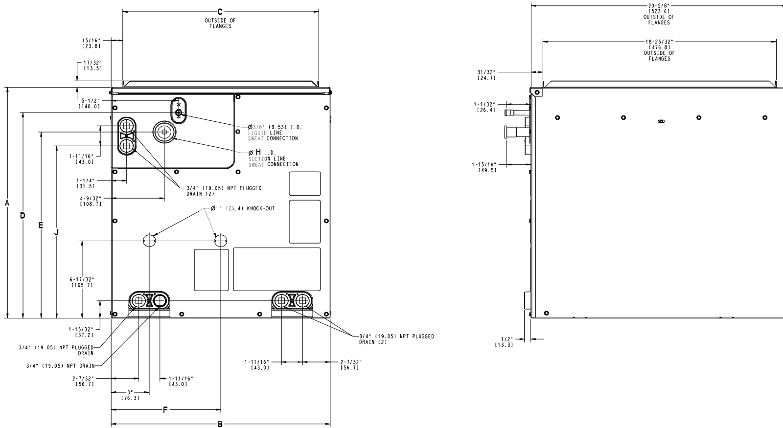
Fig. 9 – EVM4X Dimensions
