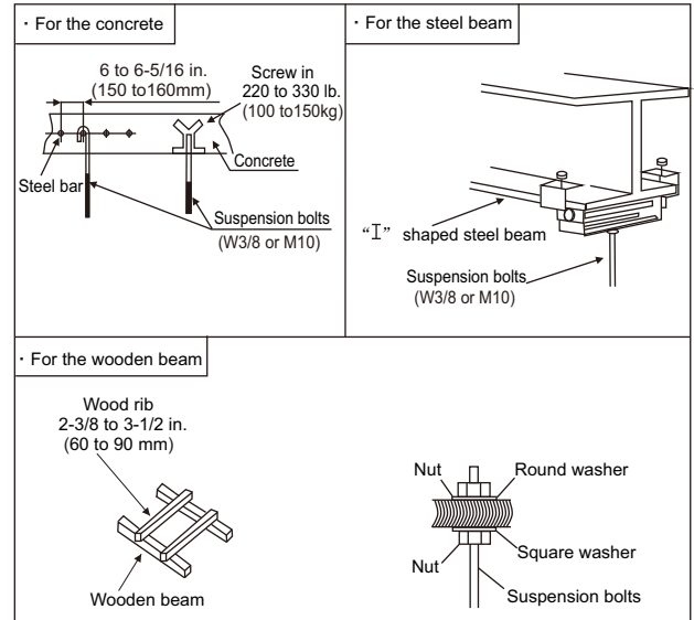
Fig. 3.2.1 Securing the suspension bolts
