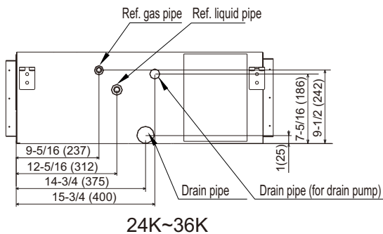
Fig. 4.1 The connection positions of the pipe
