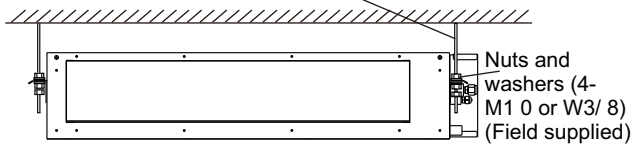
Fig. 3.4 The installation of the indoor unit
