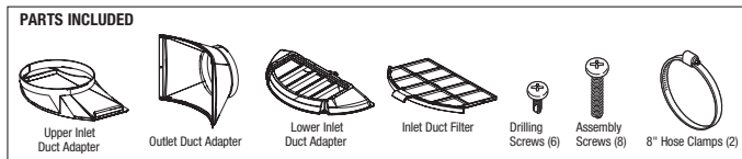
Optional Ducting Kit: Part No. 415-52820-00. Kit installation also requires - 8" (203mm) insulated flexible ducting, ducting support hangers and exterior wall vents for inlet & outlet. Additional clearances required for ducting, refer to ducting kit instructions.
