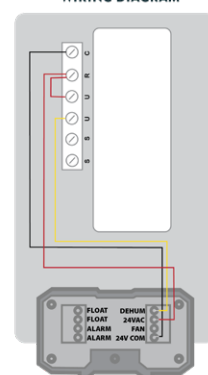
4041649 HONEYWELL HUMIDIPRO WIRING DIAGRAM
